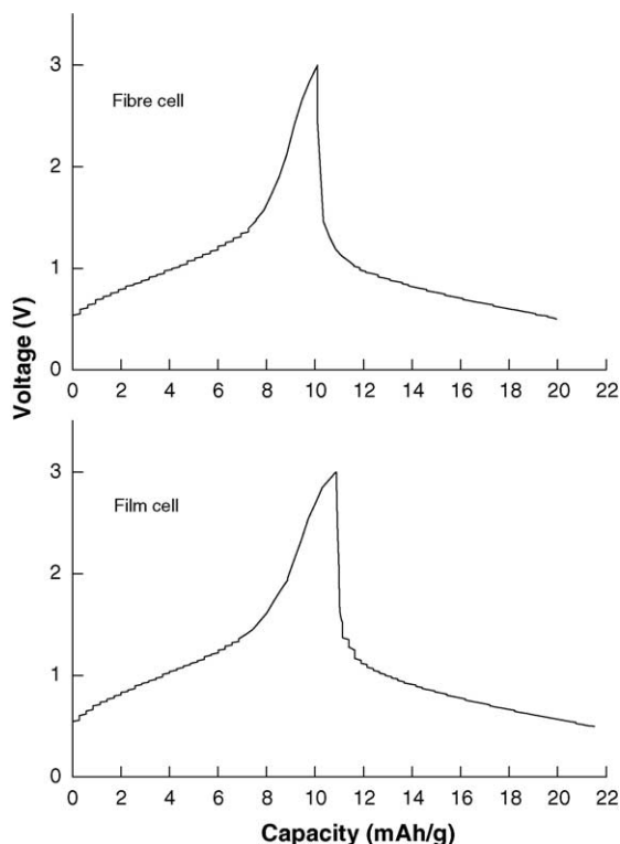
Fig. 6. Charge–discharge curves for fibre cell and film cell of PPy/LiPF 6 |EC–DMC|PPy/PSS; current density = 0.1 mA h cm -2 .
