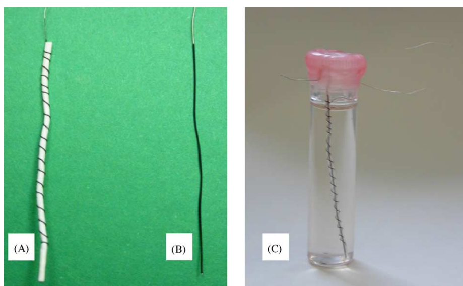
Fig. 3. Photographs of: (A) PPy/PSS/Pt wire–PVDF hollow fibre membrane composite anode; (B) PPy/PF 6 -coated Pt wire cathode; (C) test cell of PPy/PF 6 wire|LiPF 6 –EC–DMC|PPy/PSS–PVDF hollow fibre membrane composite.
