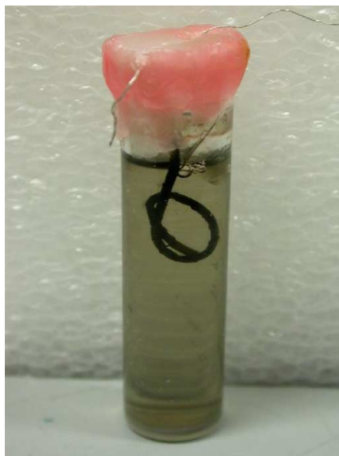
Fig. 8. Photograph of knotted fibre battery.
